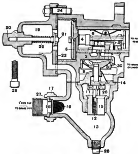
Fig. 2490. Quick-Action Triple Valve, Type P.
